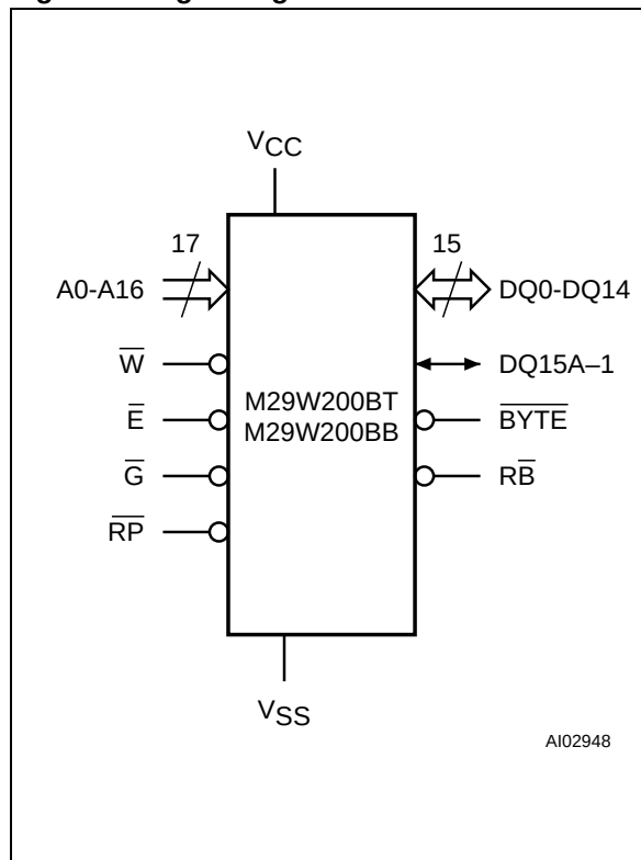
Figure 1. Logic Diagram
